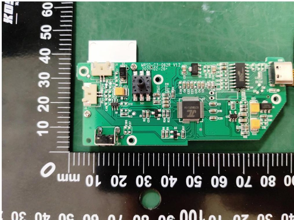
Figure 7. Top view of PCB
