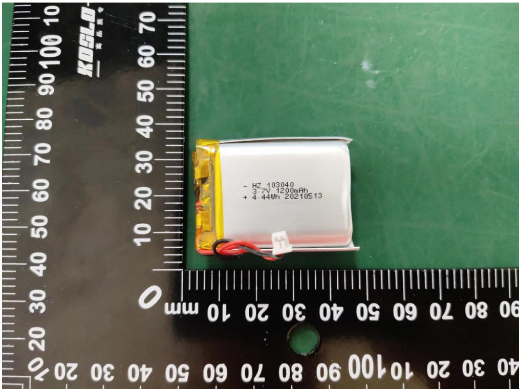
Figure 6. Overall view of Battery
