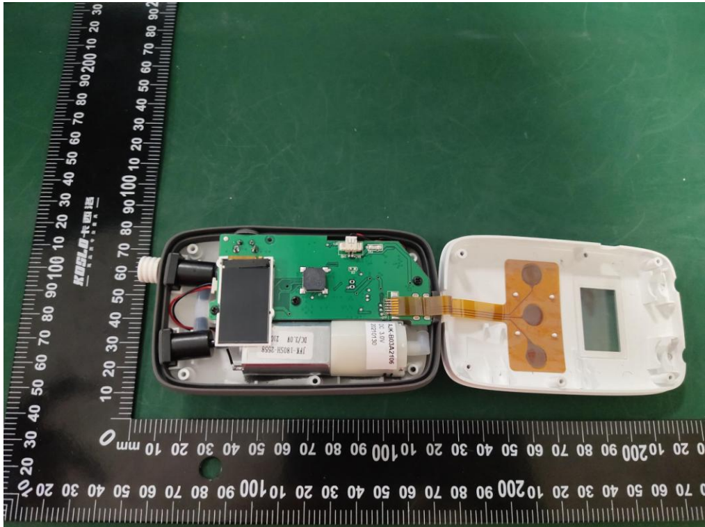
Figure 3. Internal view of unit
